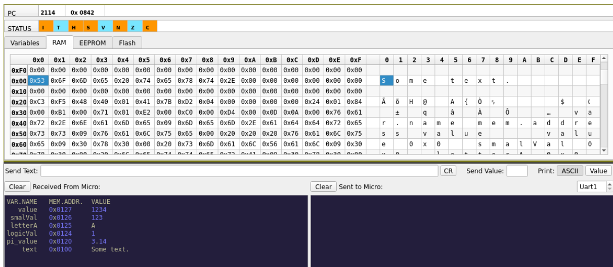
Figure 5.1: Table of values stroed in RAM memory of Arduino UNO controller.
