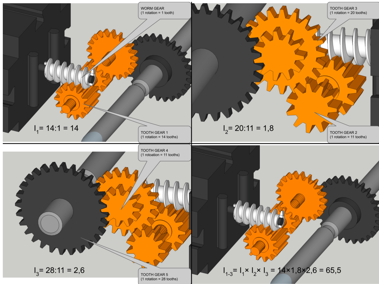
Figure 3.4: Gear ration calculation.
