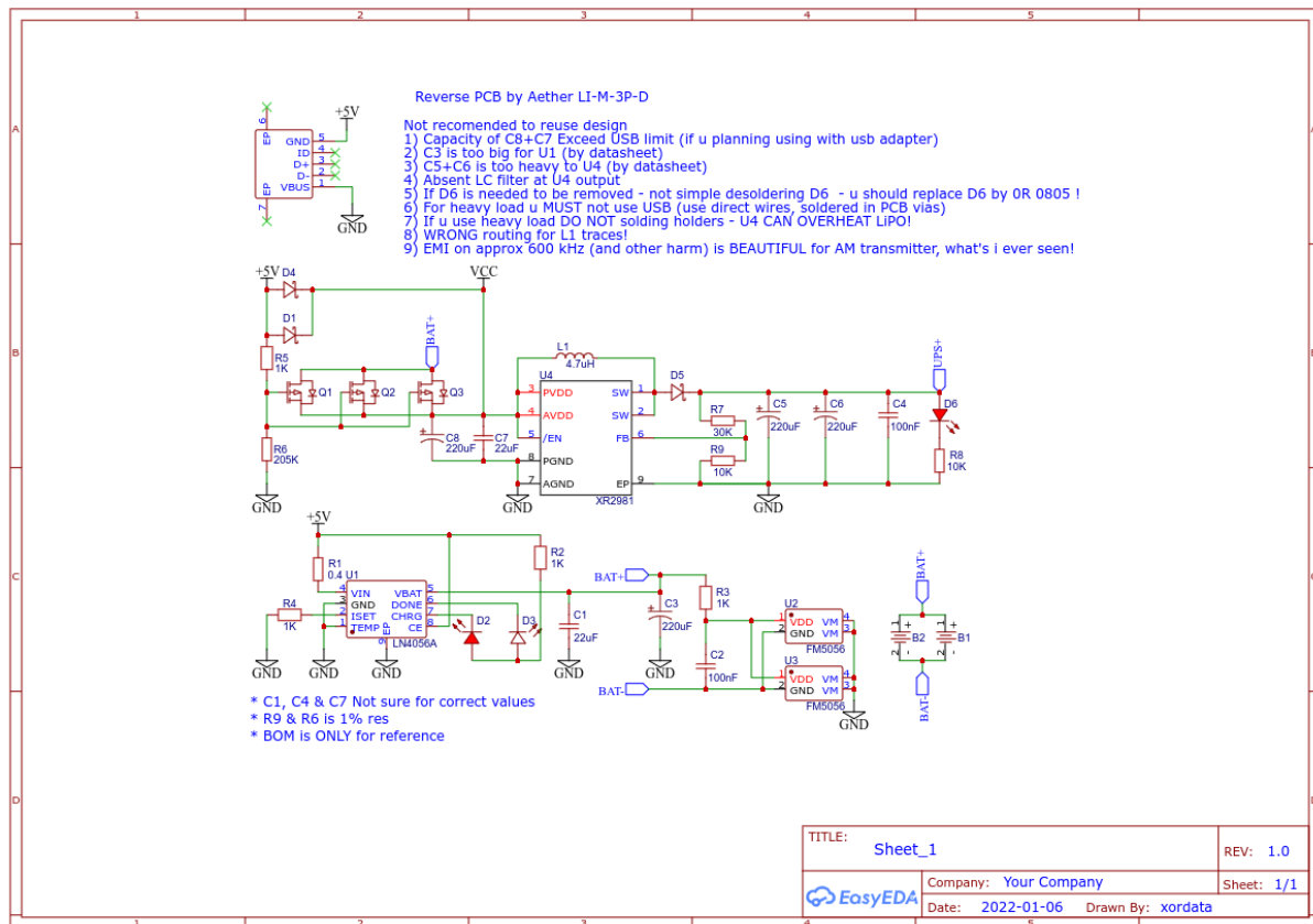
Figure 4.2: Schematic of UPS 2 .
