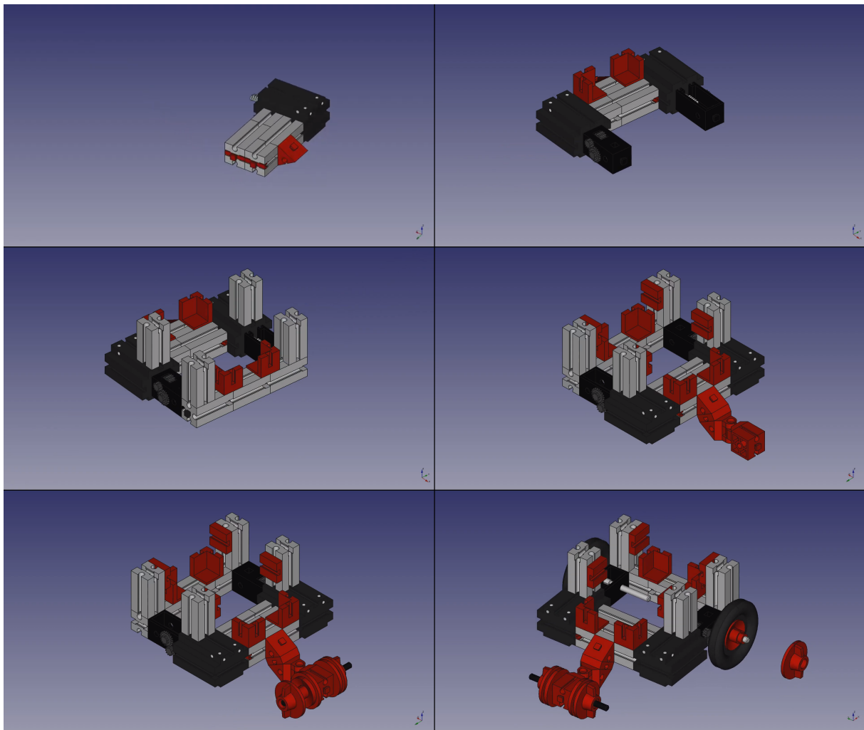
Figure 3.5: Construction sequences.
