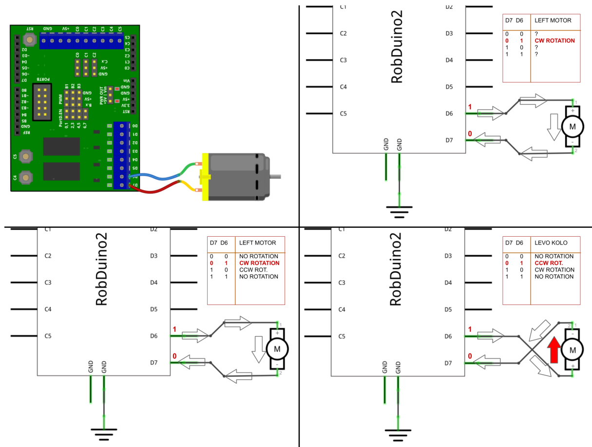
Figure 3.2: Wiring the DC motor to controller.
