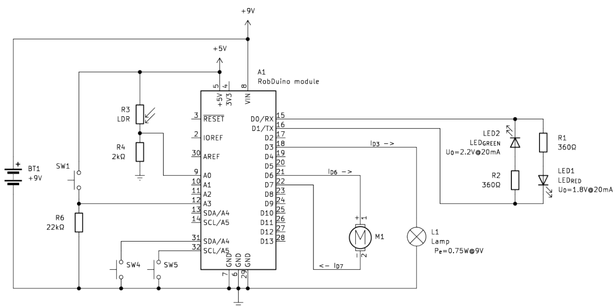
Figure 4.5: Scheme of robotic device.
