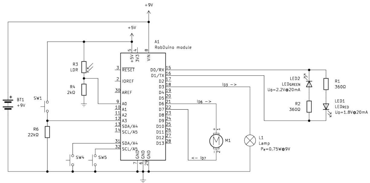
Figure 4.4: Electrical scheme of robotic device.
