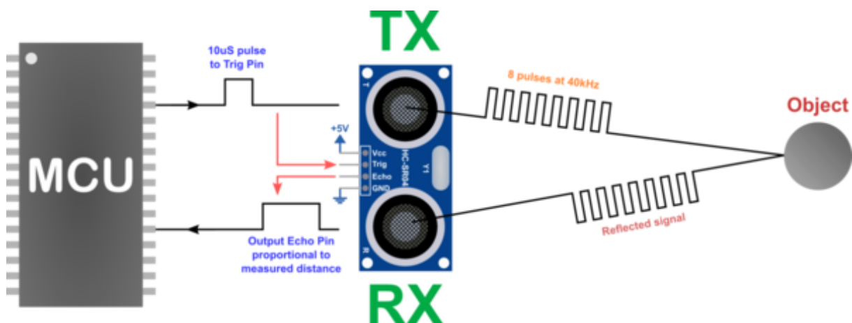
Figure 6.3: How Ultrasonic sensor works.
