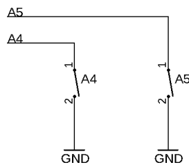
Figure 6.2: Wiring of on-board switches.
