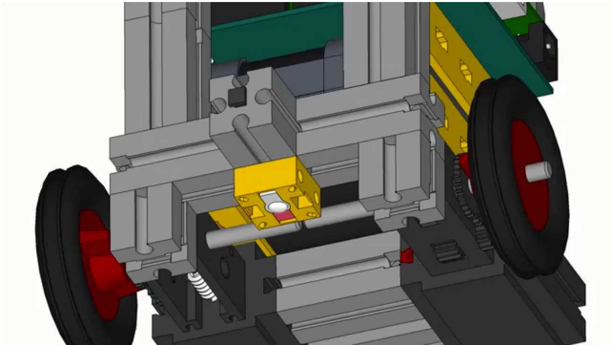
Figure 6.5: Mounting a light sensor.
