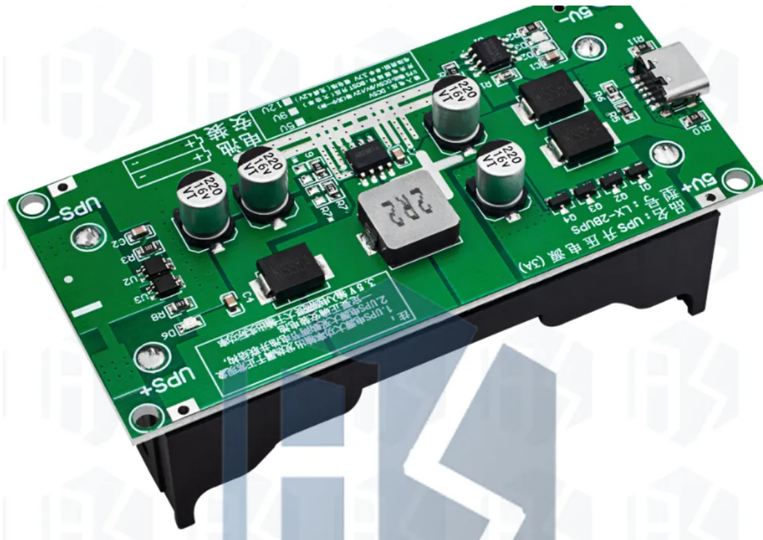
Figure 4.1: UPS power supply 1 .
